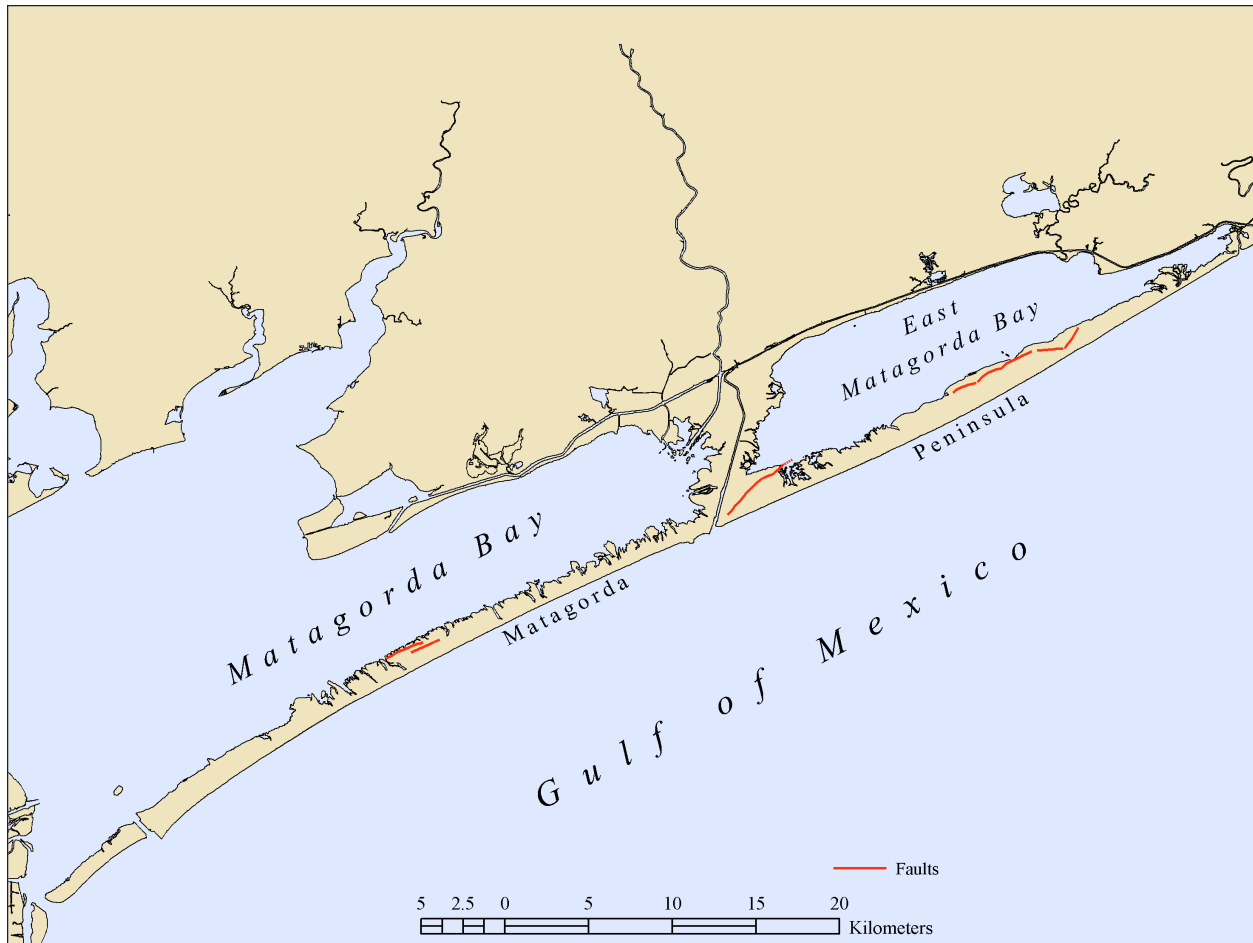
Figure 26. Index map of active faults that intersect wetlands on Matagorda Peninsula. These faults were identified and mapped using 2001 aerial photographs.
