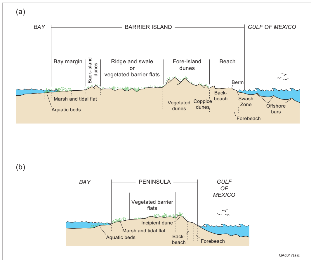
Figure 3. Schematic profiles across (a) Matagorda Island and (b) Matagorda Peninsula illustrating major environments. Not drawn to scale.
